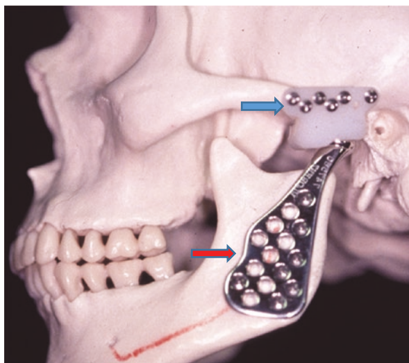
Fig. 9.3 Photograph of Zimmer Biomet stock total joint prosthesis with fossa component ( blue arrow ) and mandibular component ( red arrow )
